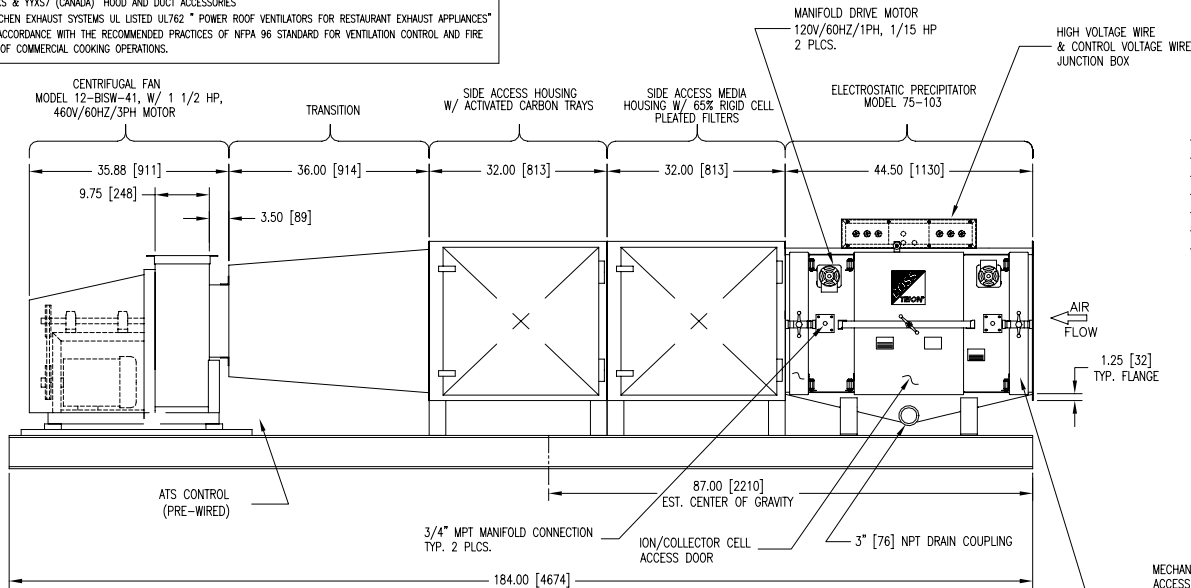
ELEVATION VIEW
