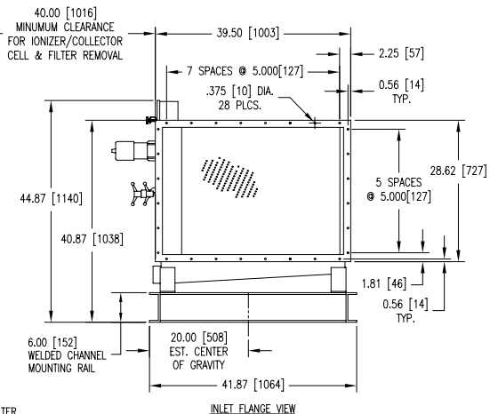
INLET FLANGE VIEW
