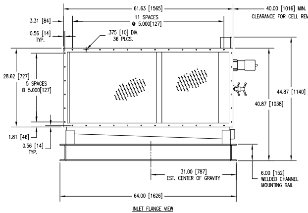
INLET FLANGE VIEW
