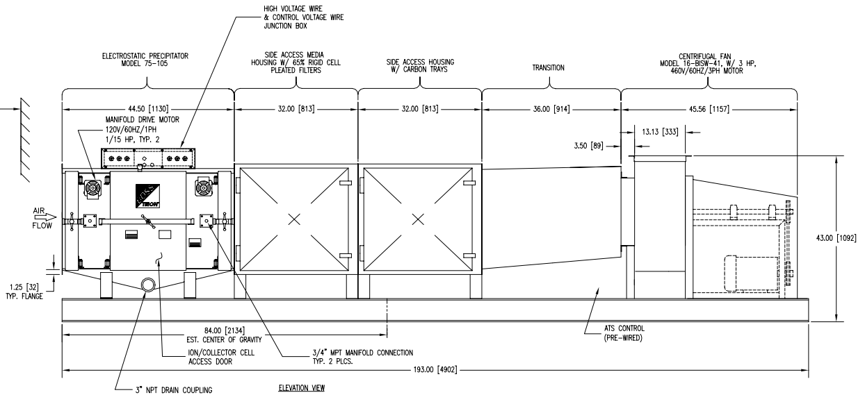
ELEVATION VIEW
